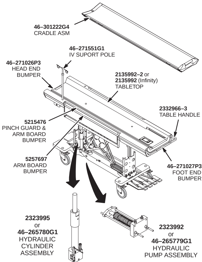
PATIENT SUPPORT TABLE
